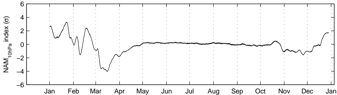
NAM 10hPa index updated: 31-Dec-2016
